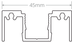
45.01 Mullion
