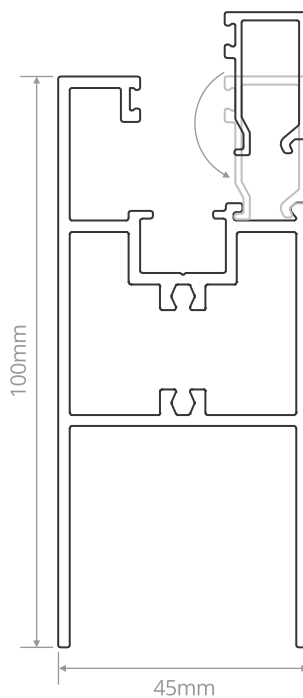
SD 80.02 45mm Door Stile Horizontal
